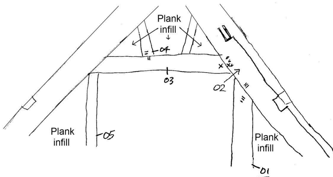
Figure 1: Sketch of the south face of the truss in room ‘Artro’ – showing the timbers sampled
