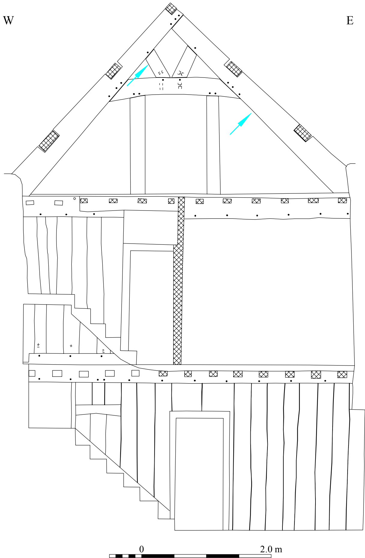
Figure 7: Truss 2 and Post and Panel Partition Scale 1:35
