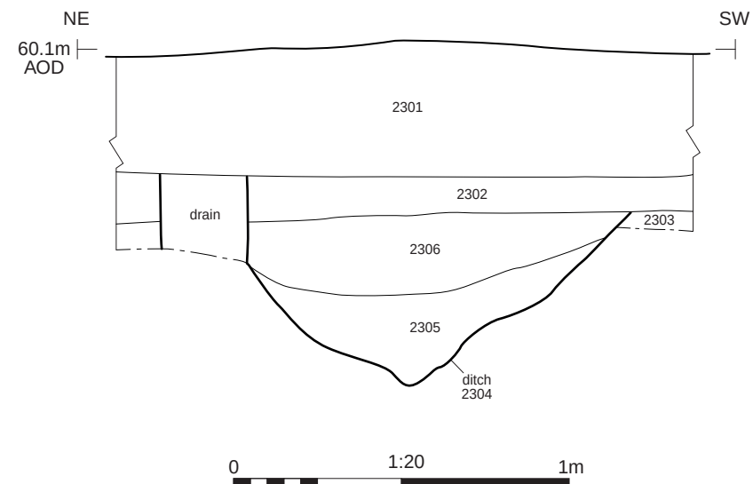
Section BB
