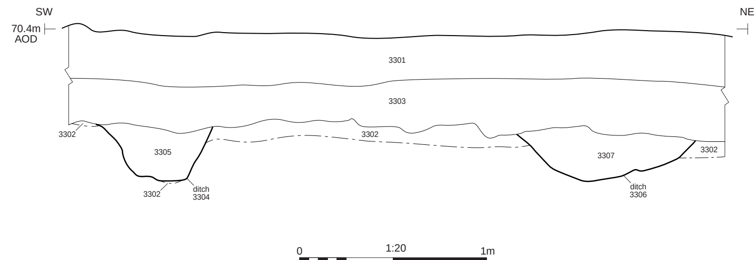
Section CC
