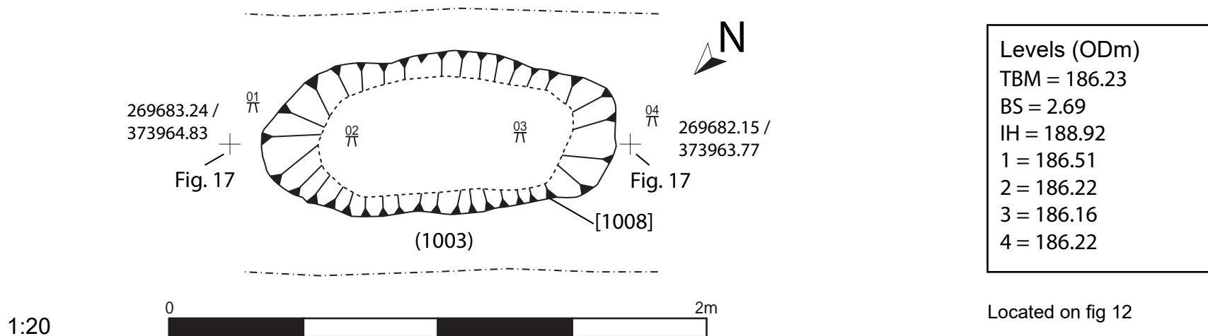
Figure 18: Plan of pit [1008], scale 1:20 at A4.
