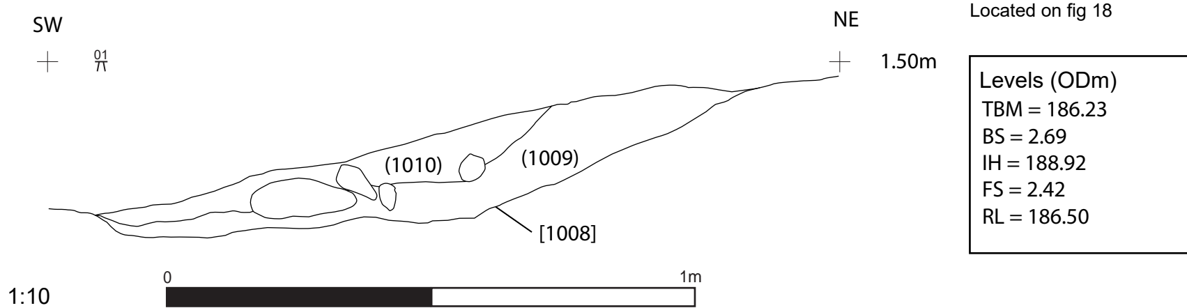
Figure 17: Southeast facing section of pit [1008], scale 1:10 at A4.
