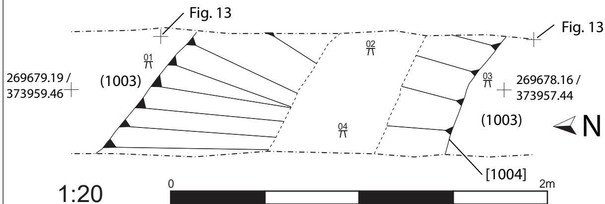
Figure 16: Plan of ditch [1004], scale 1:20 at A4.
