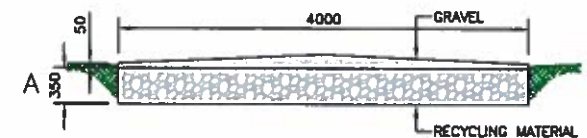
ACCESS ROAD CONSTRUCTION DETAIL SECTION A-A (1:50)
