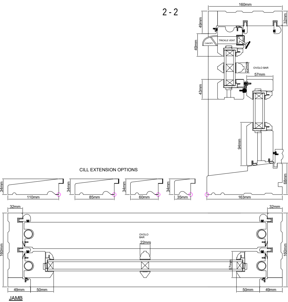
45° BAY POST CONSERVATION SPRING SASH
