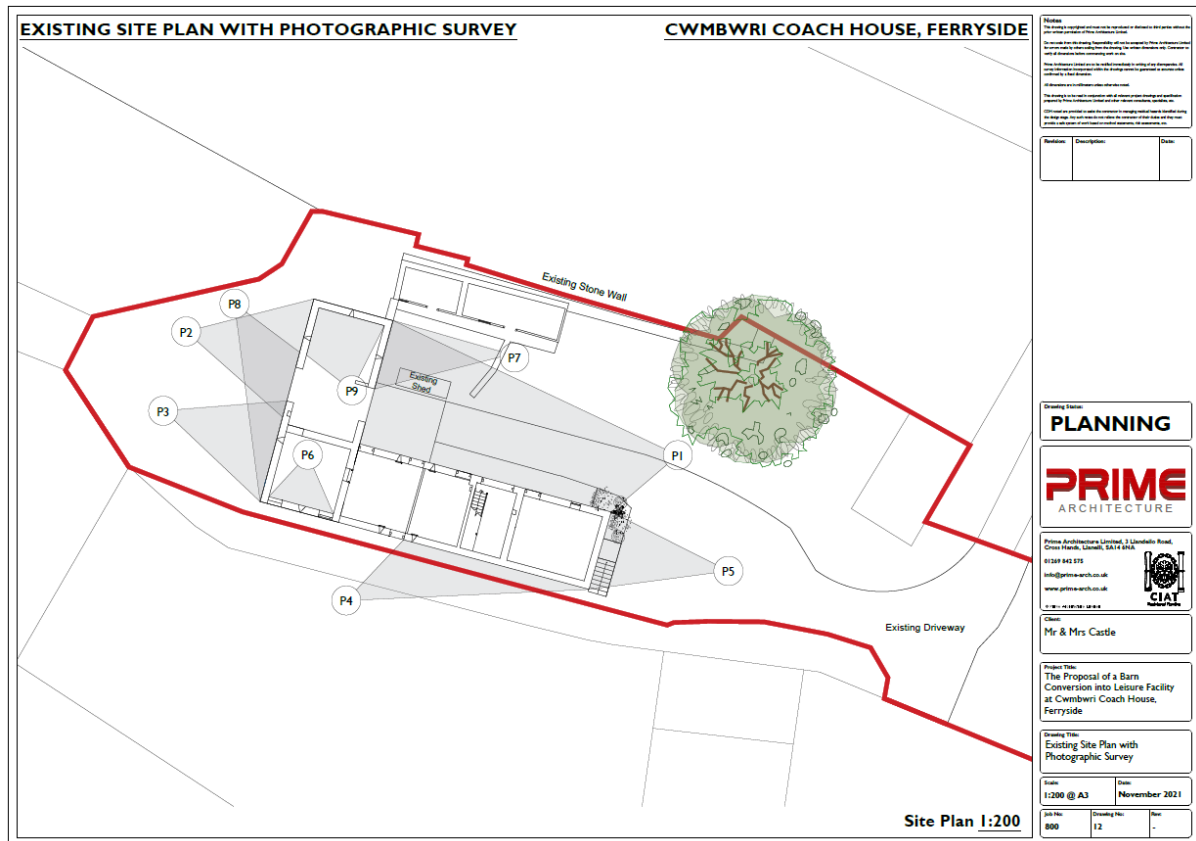
Existing Site Plan with Photographic Survey
