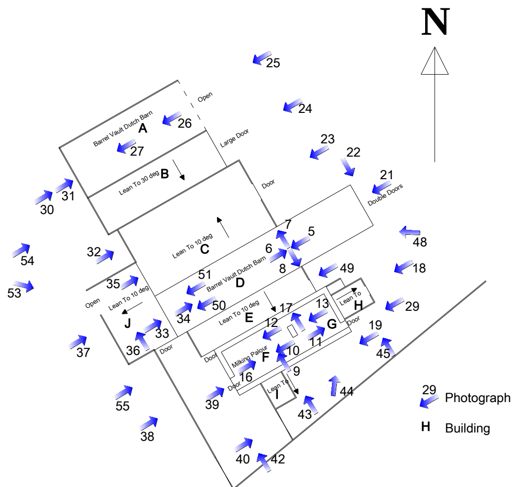
Plan of Building Showing Location Of Photographs
