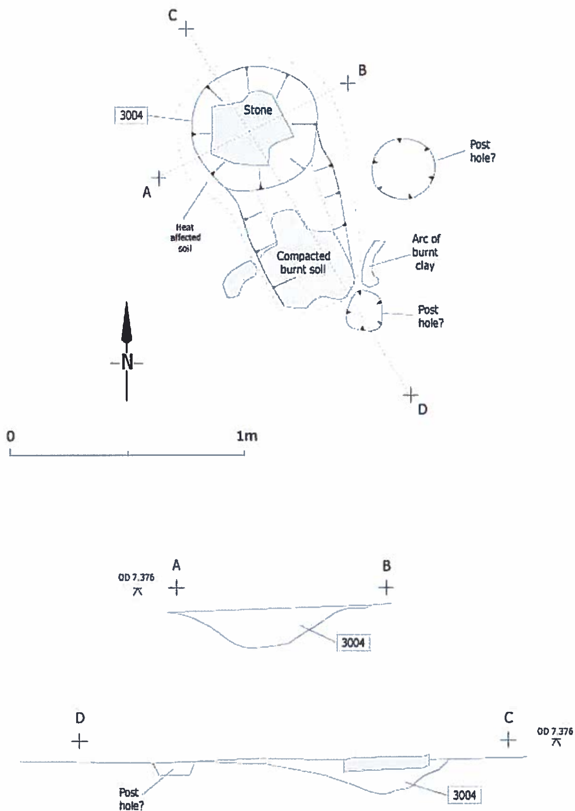
Figure 11: Plans and sections of possible Bloomery furnace [3004]
