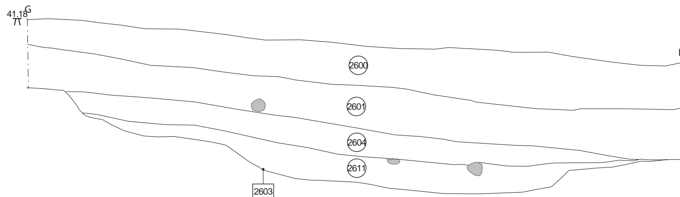
East facing section of Ditch [2603] within Trench 26
