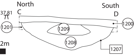
West facing section of [1207] in Trench 12
