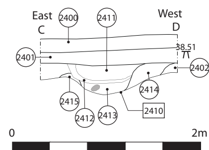
North facing section of [2410] in Trench 24
