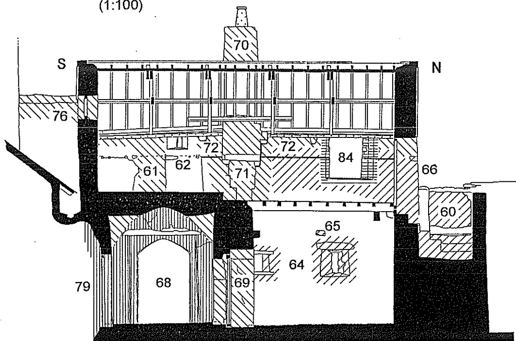
E.17: Interior elevation of the east face of the Western Range (1:100)
