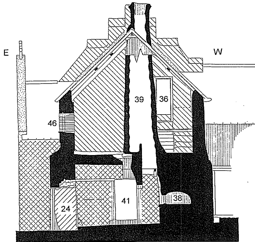
E.13: Section through the Eastern Range at first floor dividing wall looking south (1:100)
