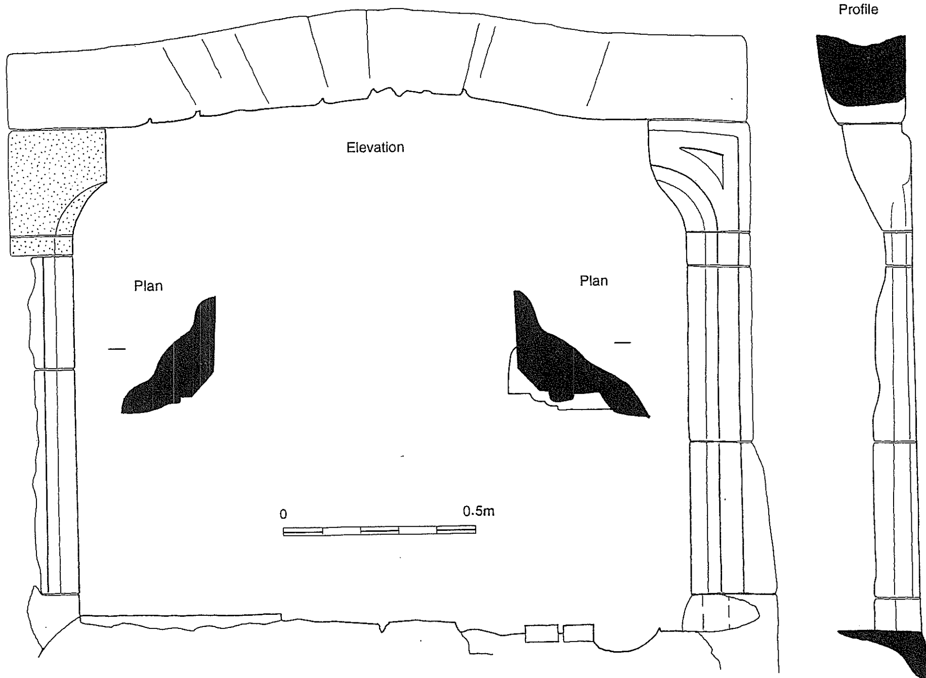
D.5: Fireplace (32), Eastern Range (1:10)
