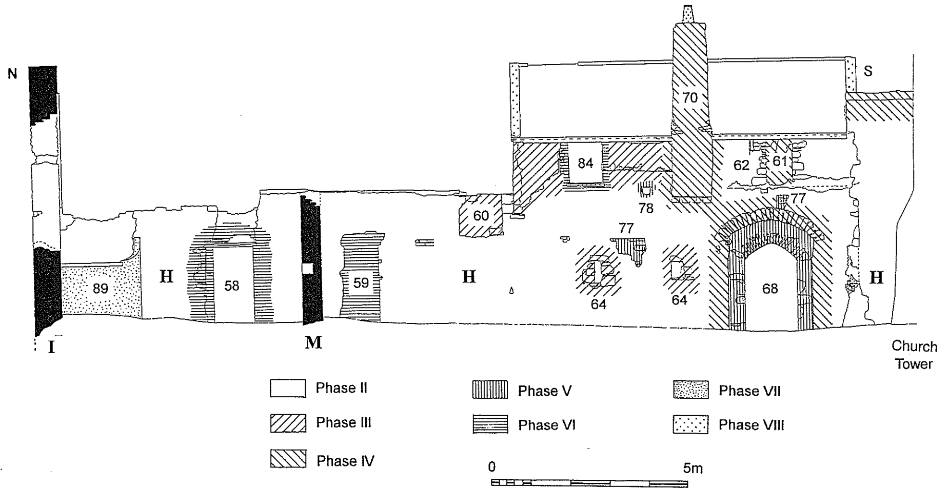
E.15: Exterior elevation of the west face of the Western Range (1:200)
