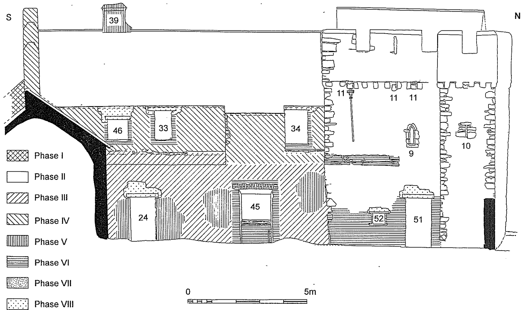
E.4: Exterior elevation of the east face of the Eastern Range and Tower (1:100)
