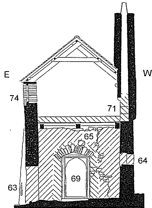
E.22: Section through the Western Range at ground floor dividing wall looking south (1:100)
