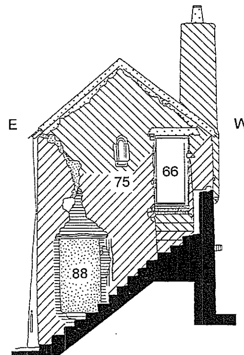
E.20: Exterior elevation of the north face of the Western Range (1:100)
