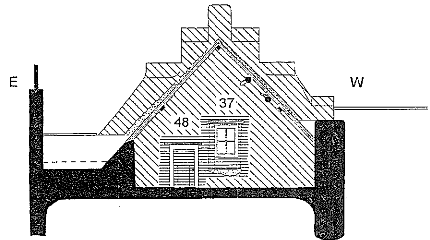
E.14: Interior elevation of the south face of the Eastern Range first floor (1:100)
