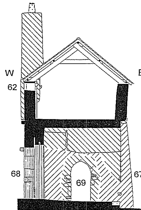
E.23: Section through the Western Range at ground floor dividing wall looking north (1:100)
