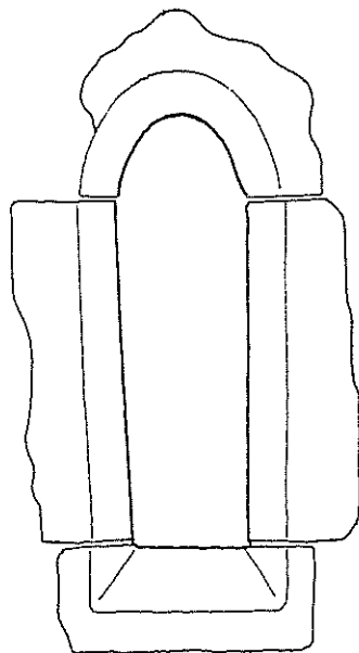
Exterior elevation
