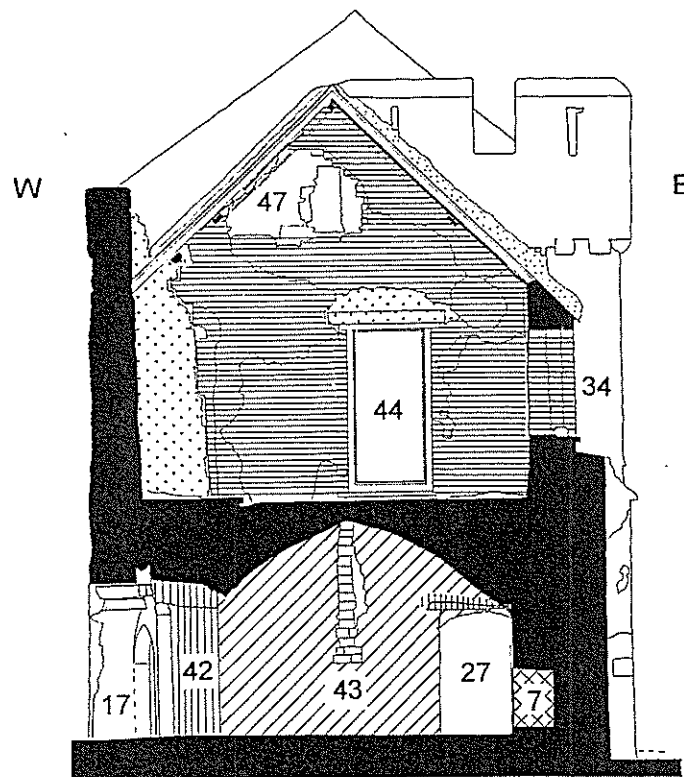
E.9: Exterior elevation of the south face of the Tower (1:100)
