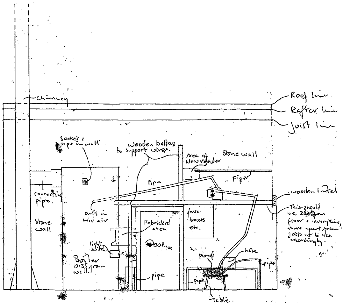
Elevation 11: East wall of Room C (boilerhouse)
