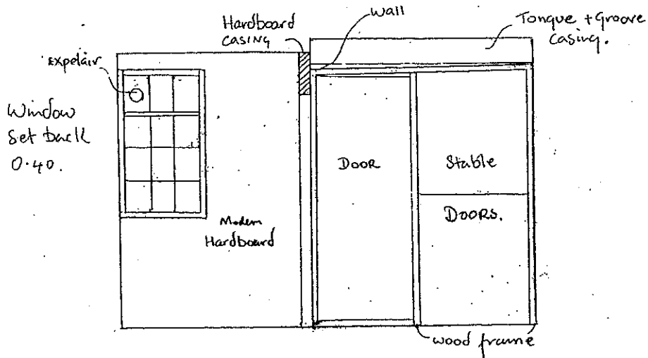
Elevation 37: East wall of Room M
