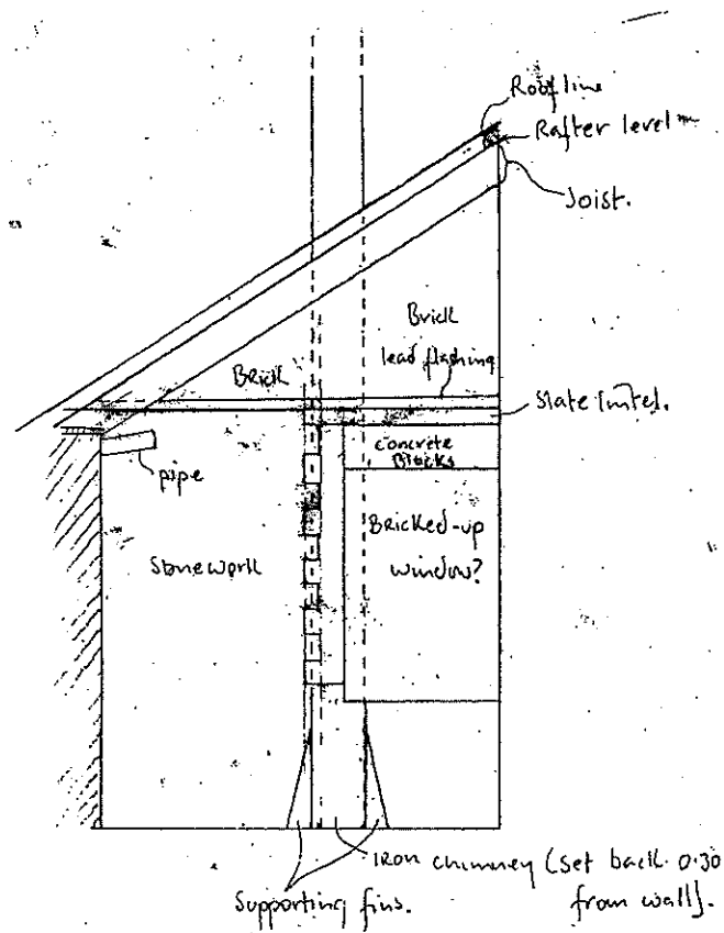
Elevation 9: North wall of Room C (boilerhouse)
