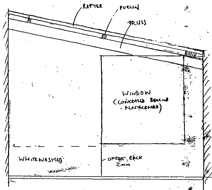
Elevation 42: West wall of Room N
