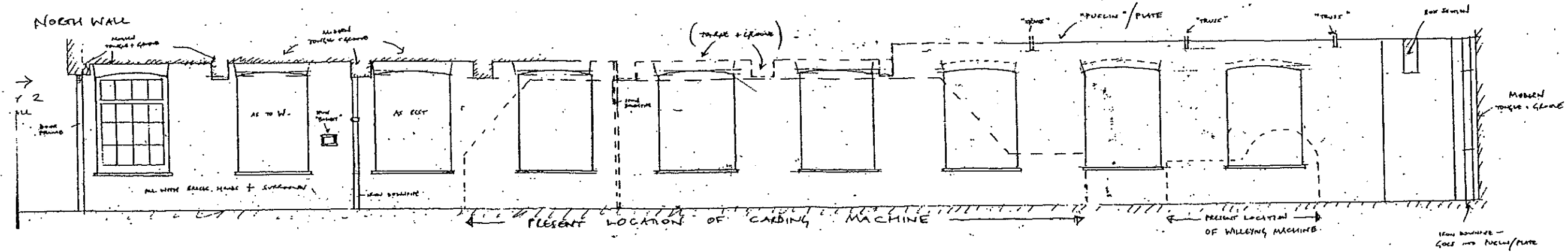
Elevation 35: North wall of Room M
