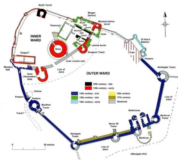
Fig. 186: Plan of Pembroke Castle
