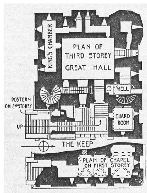
Fig. 199: The donjon at Newcastle-upon-Tyne (1170s), showing entrance stairway (plan from Toy 1963, 97)
