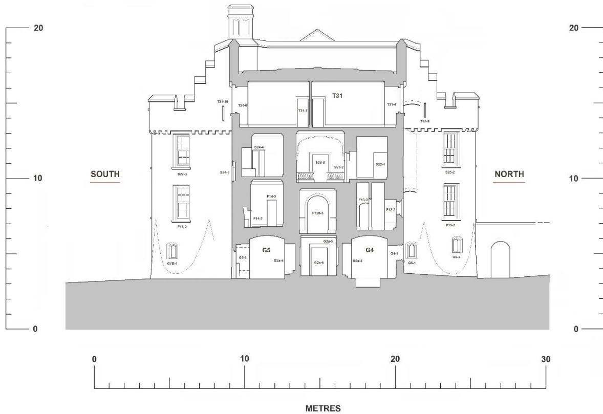
Fig. 5: Transverse section through Picton Castle east towers, facing west
