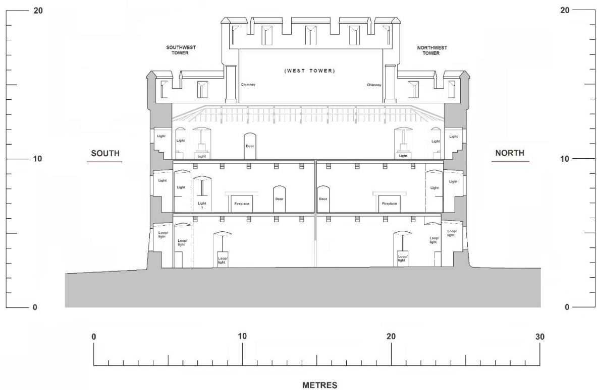
Fig. 179b: Transverse section through Picton Castle west towers, facing west – conjectured medieval
