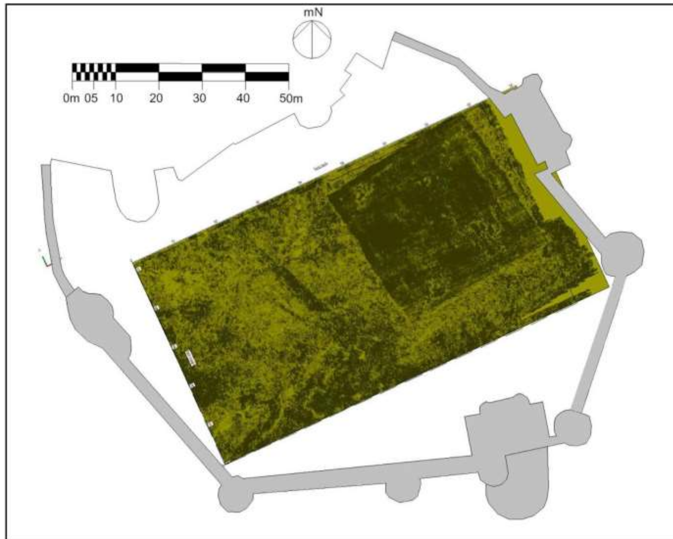
Figure 27: C-scan d= 1.1m (estimated) (from Fletcher 2016)
