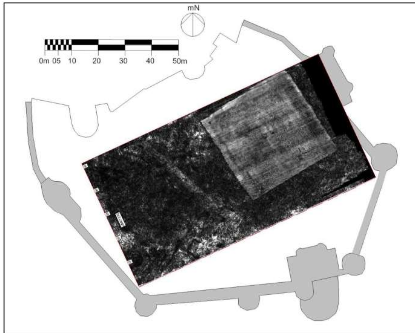
Figure 26: C-scan d= 1.0m (estimated) (from Fletcher 2016)
