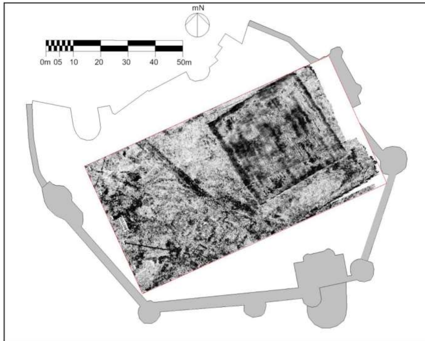
Figure 25: C-scan d= 0.35m (estimated) (from Fletcher 2016)
