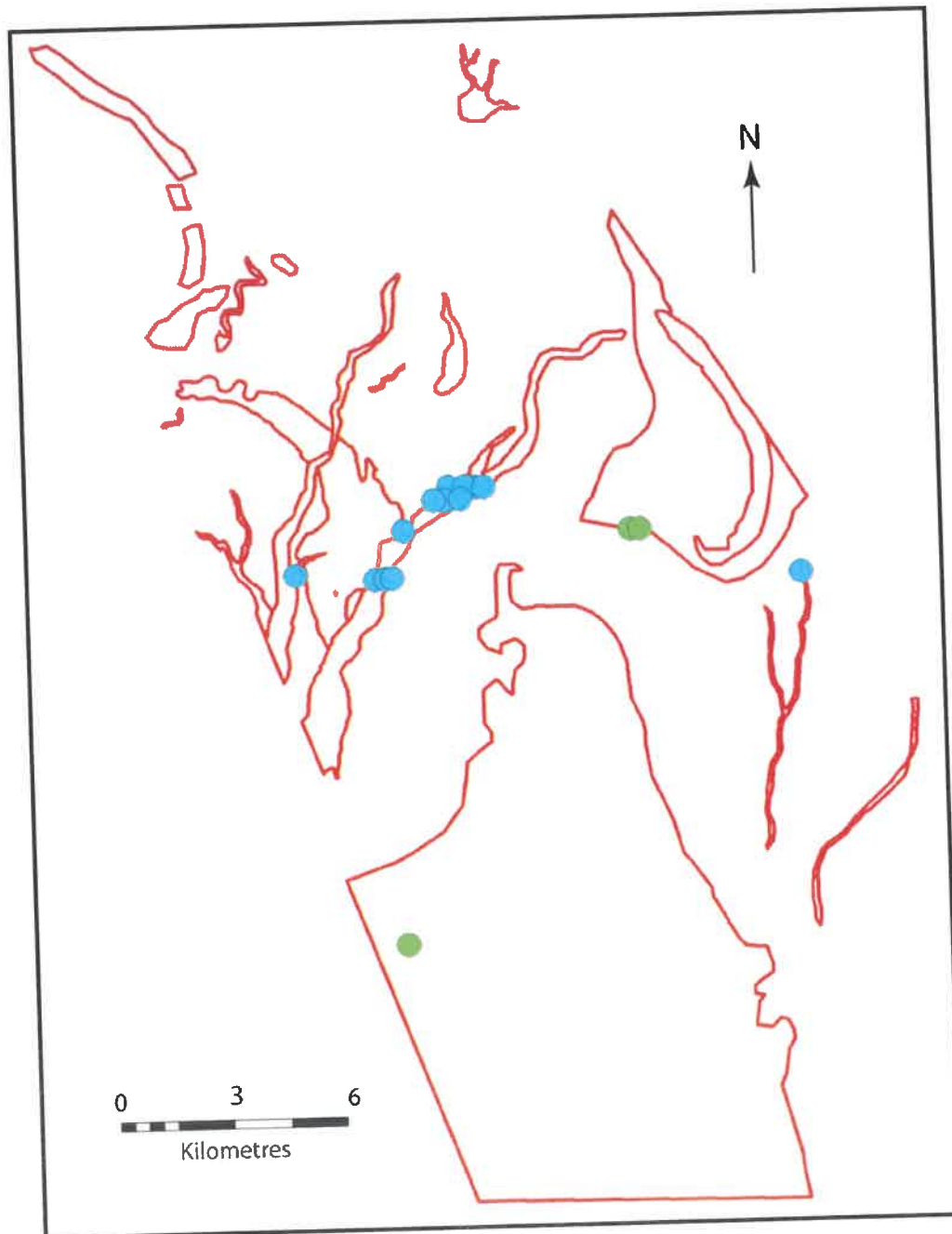
Figure 16: Observed intersections between features observed within the 3D dataset and the 2D seismic datasets. Fluvial features are given in blue. The fluvio-glacial plain is shown in green.
