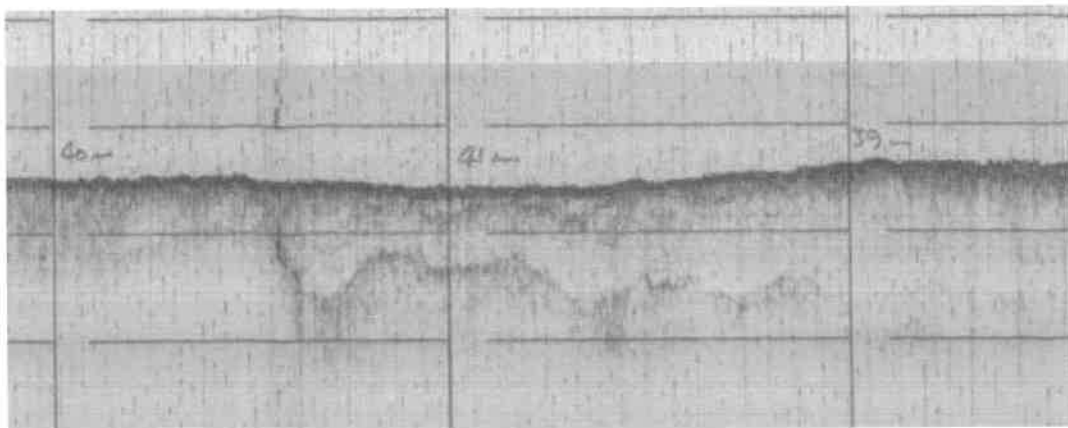
Figure 13: Palaeochannel feature located with the 1968 pinger data
