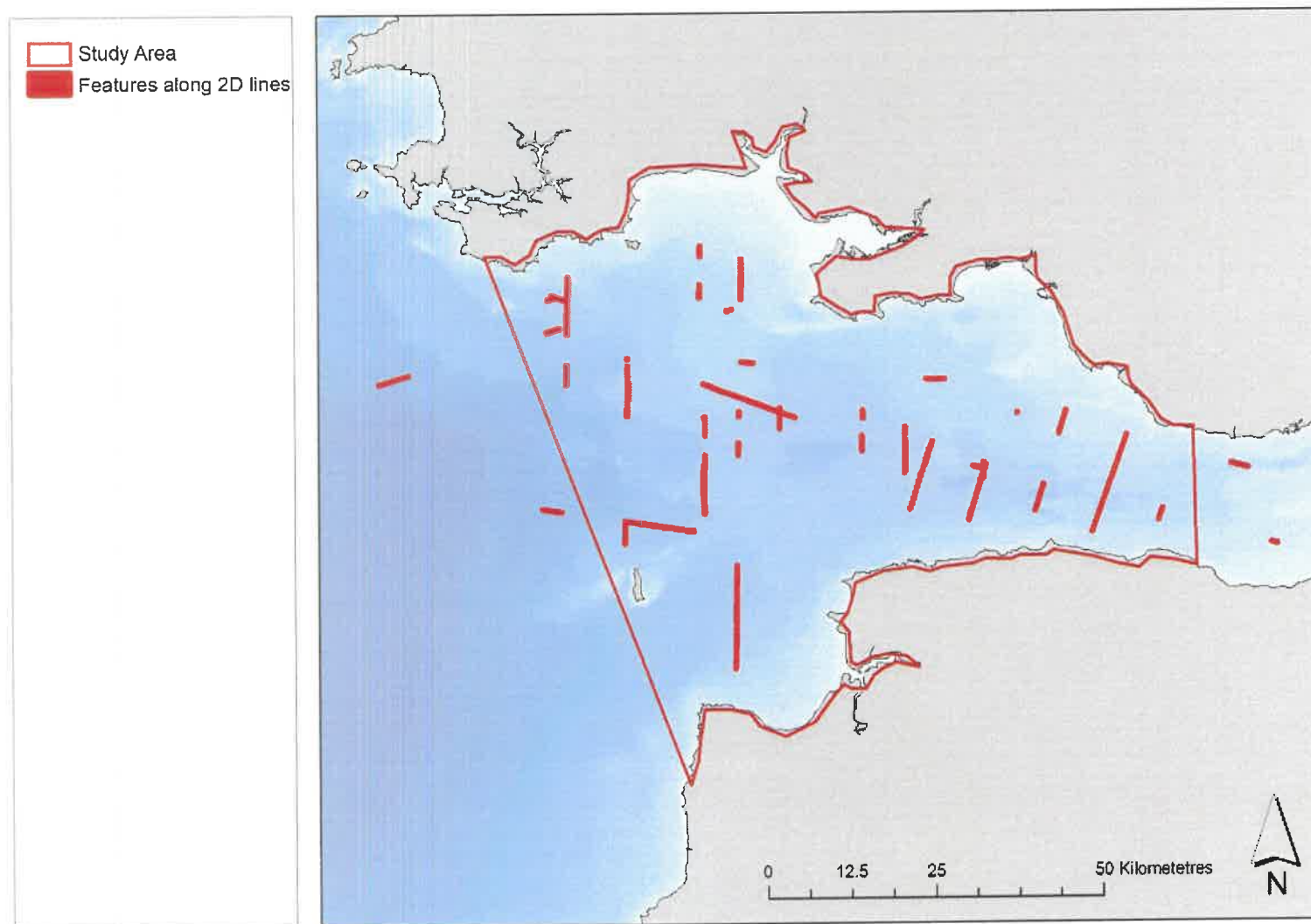
Figure 30: 2D features within the Bristol Channel study area
