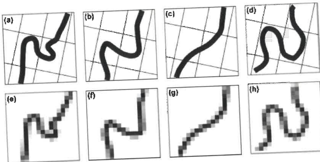
Figure 3: (a-d) Four possible interpretations of a channel morphology based on a coarse 2D seismic grid. Each interpretation is equally valid. (e-h) Schematic illustrations of how each of the interpretations shown in a-d would appear on a timeslice from a laterally continuous, binned 3D seismic volume. This demonstrates that additional information, such as 3D seismic data would be required to distinguish between the possible alternatives (after Thomson and Gaffney 2007).
