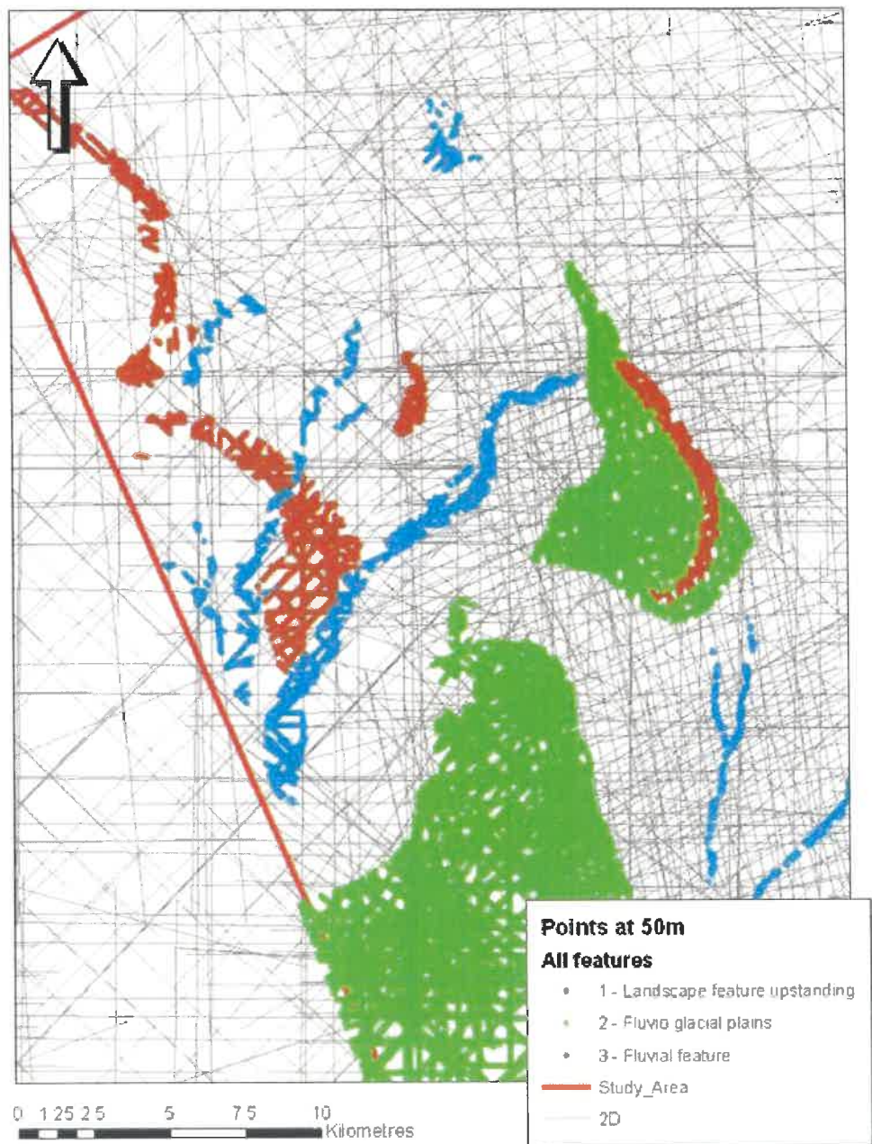
Figure 17: Results of the intersection of all of the 2D lines that intersected the features identified within the 3D seismic data
