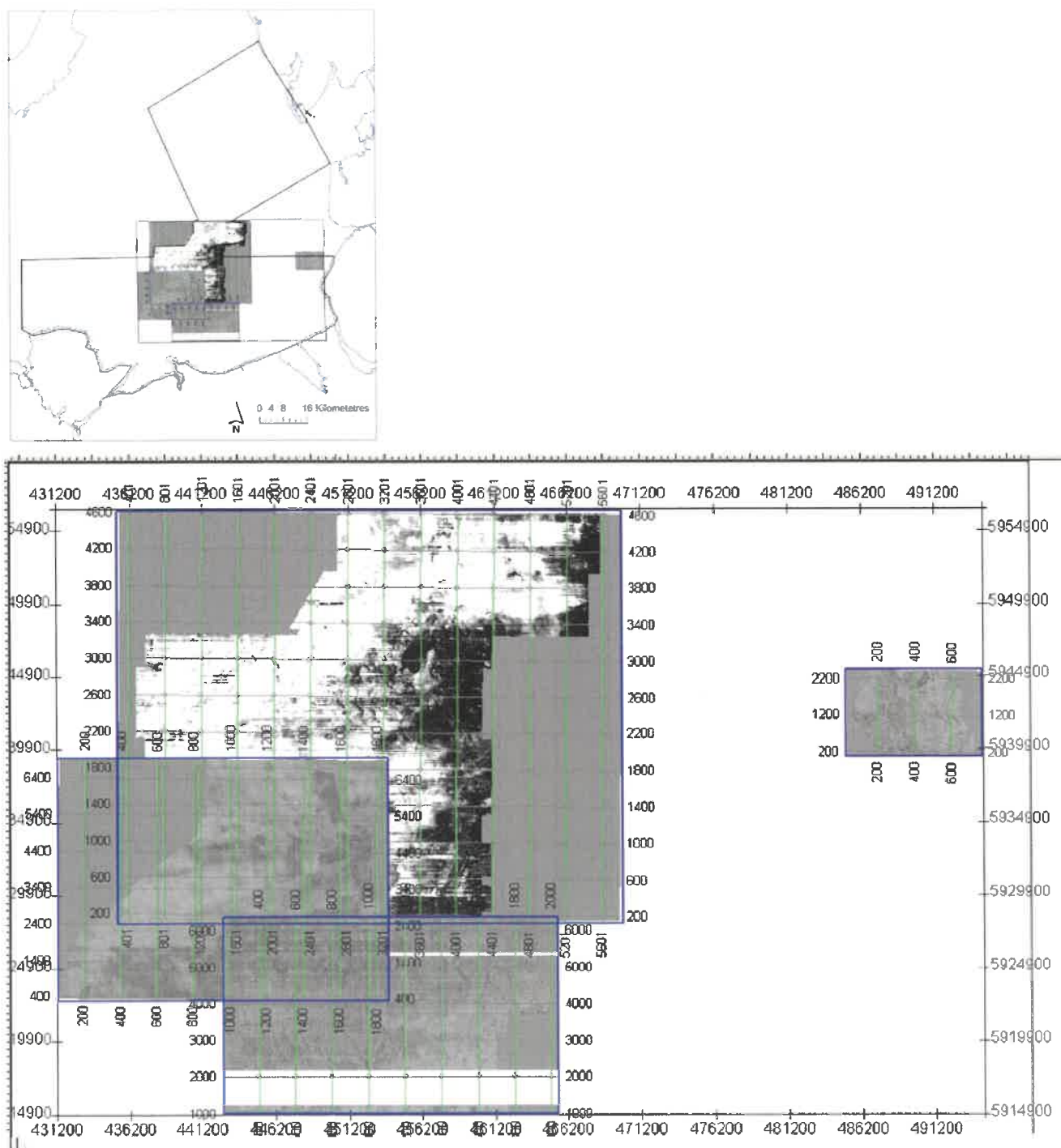
Figure 5: 3D timeslices through datasets procured within the North Wales and English marine areas (not including the Pilot Project datasets)
