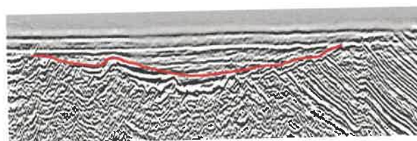
Figure 23: Sediment filled basins (example shown in red)
