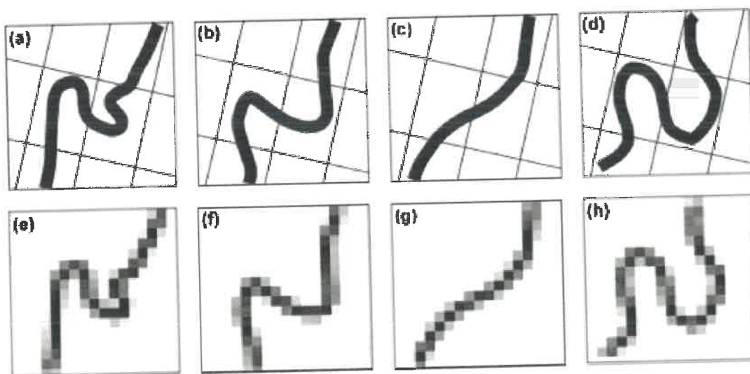
Figure 4: (a-d) Four possible interpretations of a channel morphology based on a coarse 2D seismic grid. Each interpretation is equally valid. (e-h) Schematic illustrations of how each of the interpretations shown in a-d would appear on a timeslice from a laterally continuous, binned 3D seismic volume. This demonstrates that additional information, such as 3D seismic data would be required to distinguish between the possible alternatives (after Thomson and Gaffney 2007).
